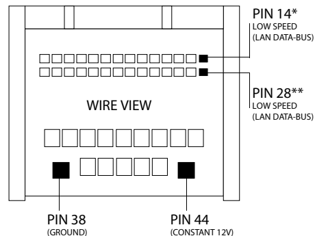
FIGURE 1: CONNECTING THE DATA-BUS WIRES
